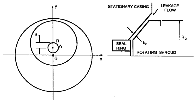
FIGURE 2a. Schematic of the whirling shroud where S is the center of the stationary casing, R is the center of the rotating shroud, W is the center of the whirl orbit along which R travels, WR = \epsilon is the eccentricity, and WS = \delta is the offset.
