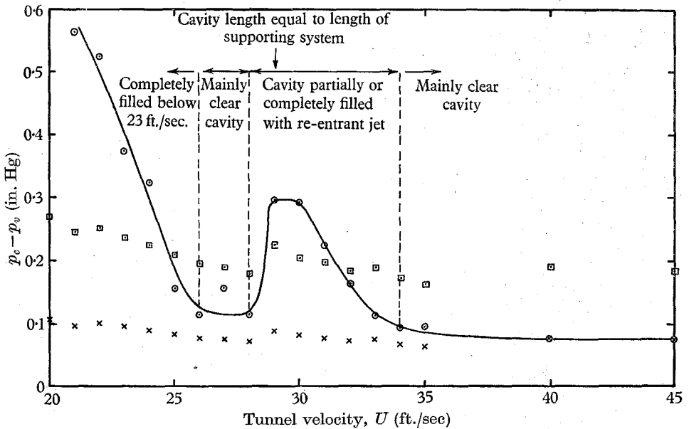
FIGURE 2. Variation of (p_c - p_v) with U , air content 9.0 p.p.m. \odot , experimental results; \square , turbulent boundary-layer theory; \times , adjusted theoretical points.
