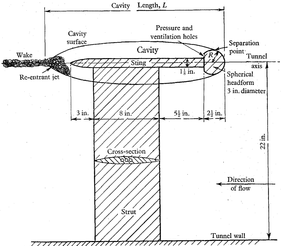
FIGURE 1. Representation of spherical headform with cavity and support system.
