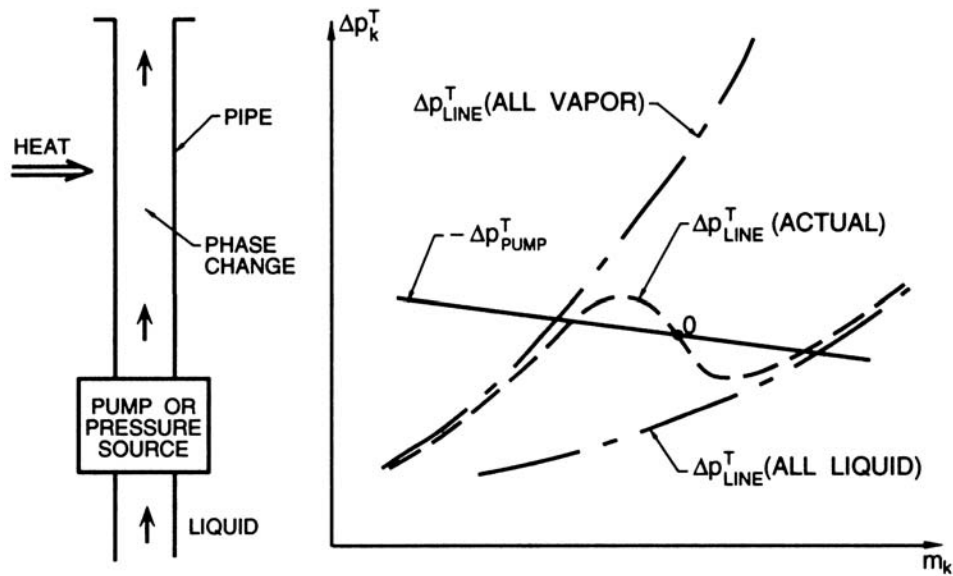
Figure 1: Sketch illustrating the Ledinegg instability.
