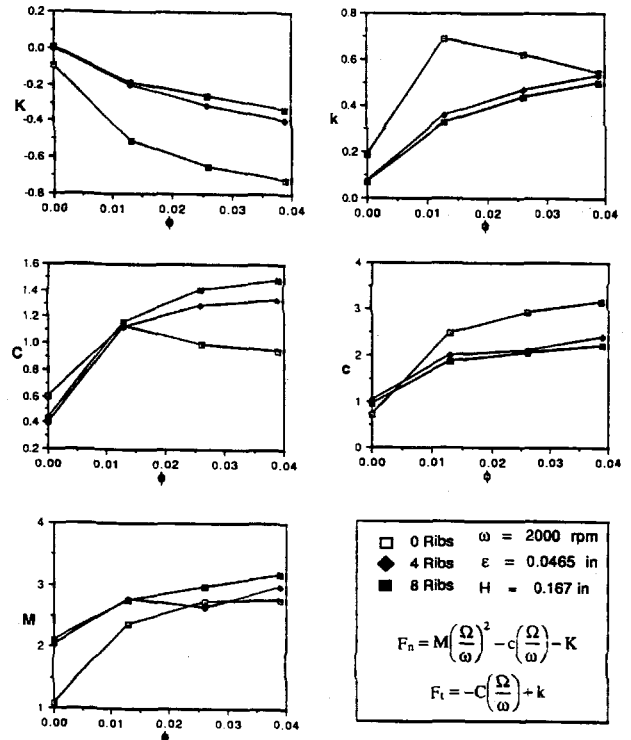
FIGURE 8. ROTORDYNAMIC COEFFICIENTS AT 2000 RPM WITH SWIRL.
