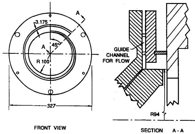
FIGURE 3. INSTALLATION OF LEAKAGE INLET SWIRL VANE. DIMENSIONS IN MM (GUINZBURG, 1992b).
