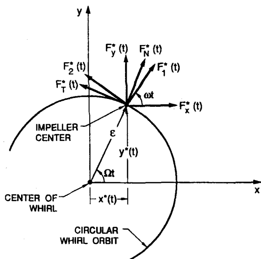
FIGURE 1. SCHEMATIC OF THE FLUID-INDUCED FORCES ACTING ON AN IMPELLER WHIRLING IN A CIRCULAR ORBIT.
