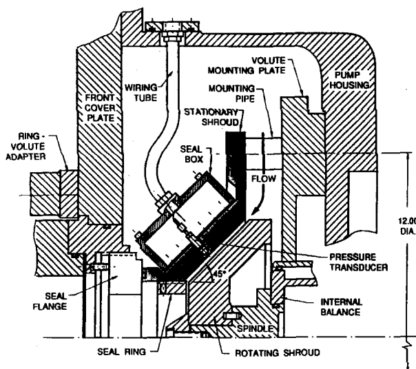
FIGURE 2. LEAKAGE FLOW TEST SECTION (ZHUANG, 1989).
